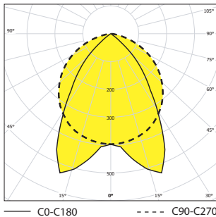
DUNKER20-4x54W, IP20
