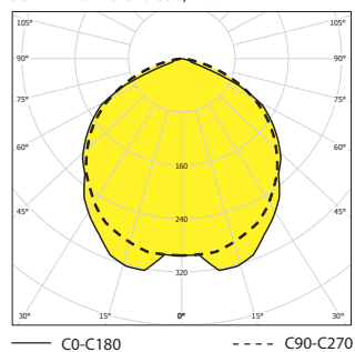
BOXER-LED-26-840-350, IP 64
