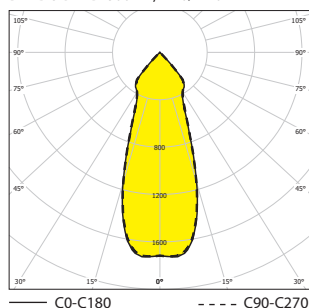
BANDOG-LED-800-4K, IP20/IP40
