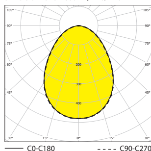
BANDOG-LED-OP-800-4K, IP20/IP40
