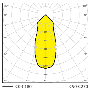
BANDOG-LED-3000-4K, IP20/IP40
